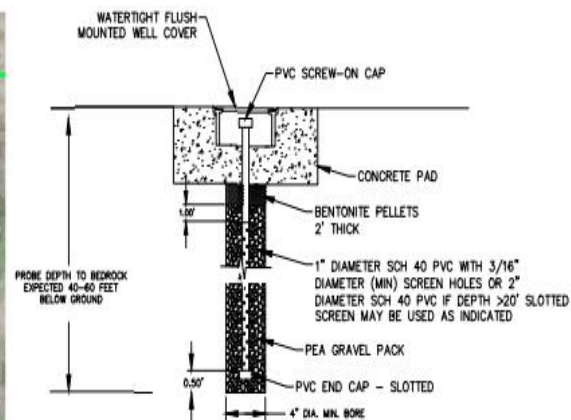
FLUSH GAS PROBE DETAIL
